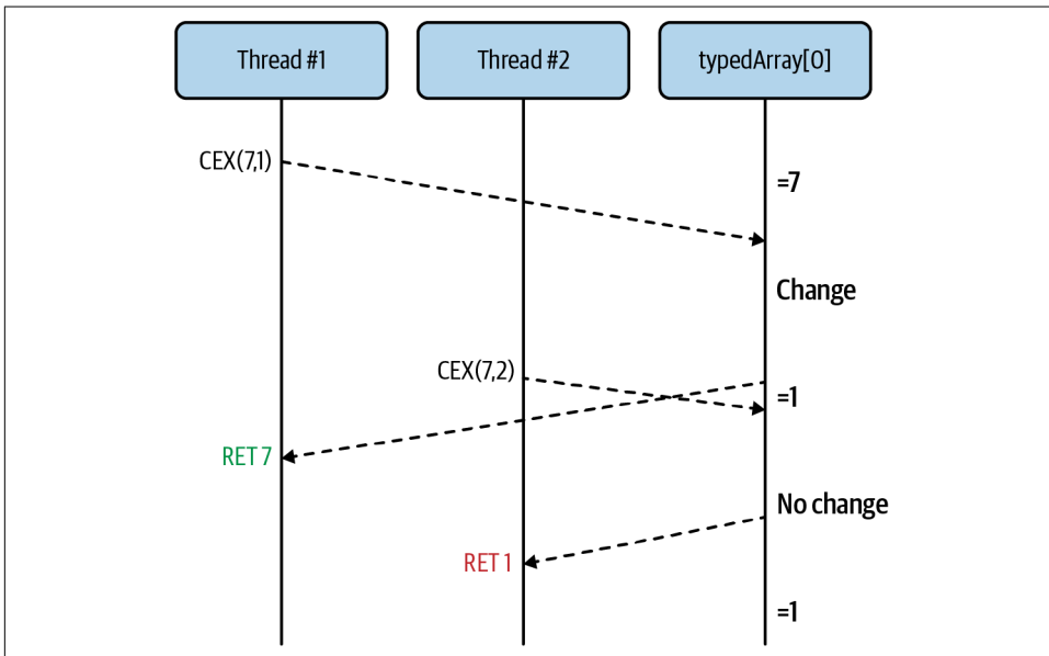
Figure 4-2. Atomic form of Atoms.compareExchange()
